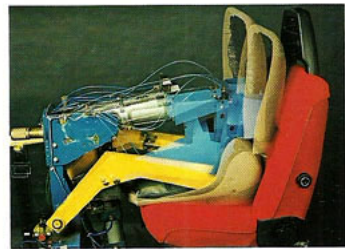
Volvo's reputation for toughness isn't just because of thick paint. Volvo also invests heavily in sophisticated testing and quality-control equipment and procedures. This machine, for instance, can put years of stress and wear on a seat in a matter of days. It represents Volvo's dedication to quality.
